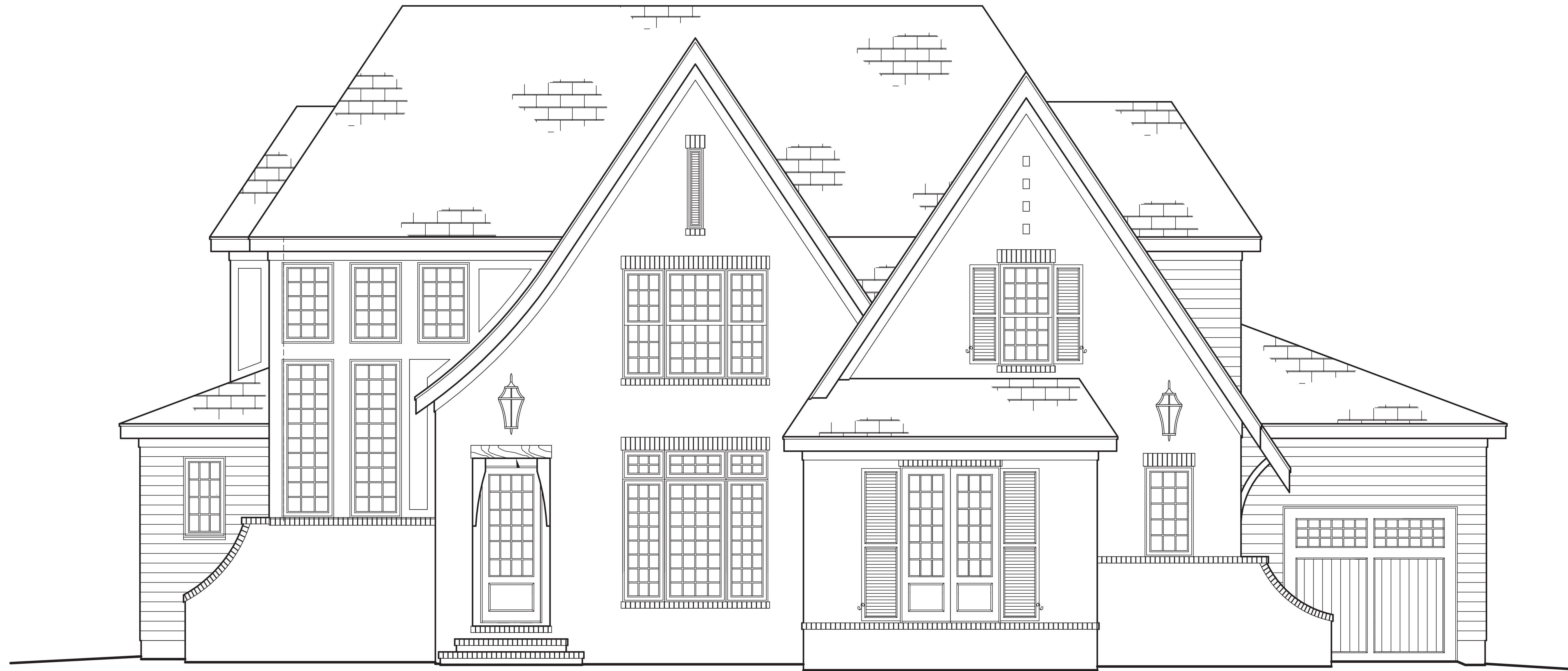
FRONT ELEVATION
